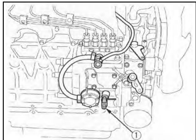
1) Ablasshahn
